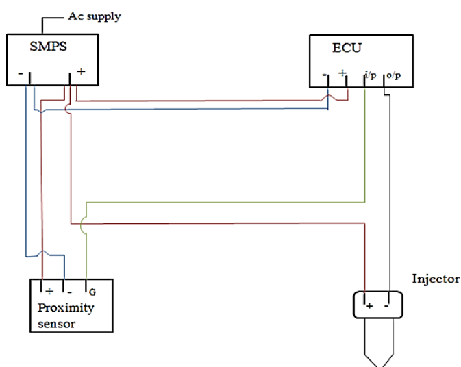
FIGURE 9. Circuit Diagram connecting ECU, Proximity sensor and injector
