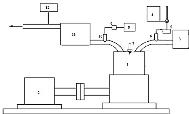
FIGURE 2. Overview of Engine setup
