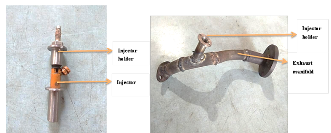
FIGURE 6. Modified Exhaust Manifold containing Injector holder
