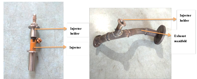
FIGURE 5. Injector with Injector Holder
