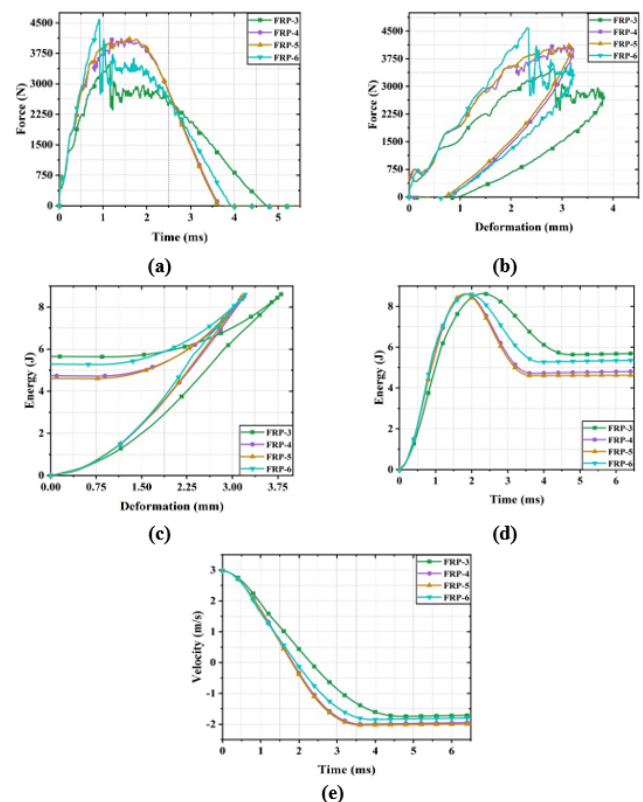
FIGURE 14. Various parameters measured during the LVI test of 40 μ SiO 2 reinforced intra-interply composites (a) Force Vs Time (b) Force Vs Deformation (c) Energy Vs Deformation (d) Energy Vs Time (e) Velocity Vs Time
