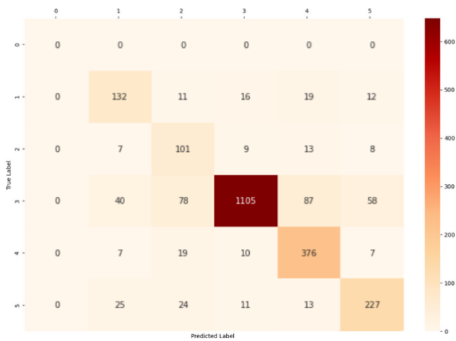
FIGURE 13. Confusion matrix after testing process
