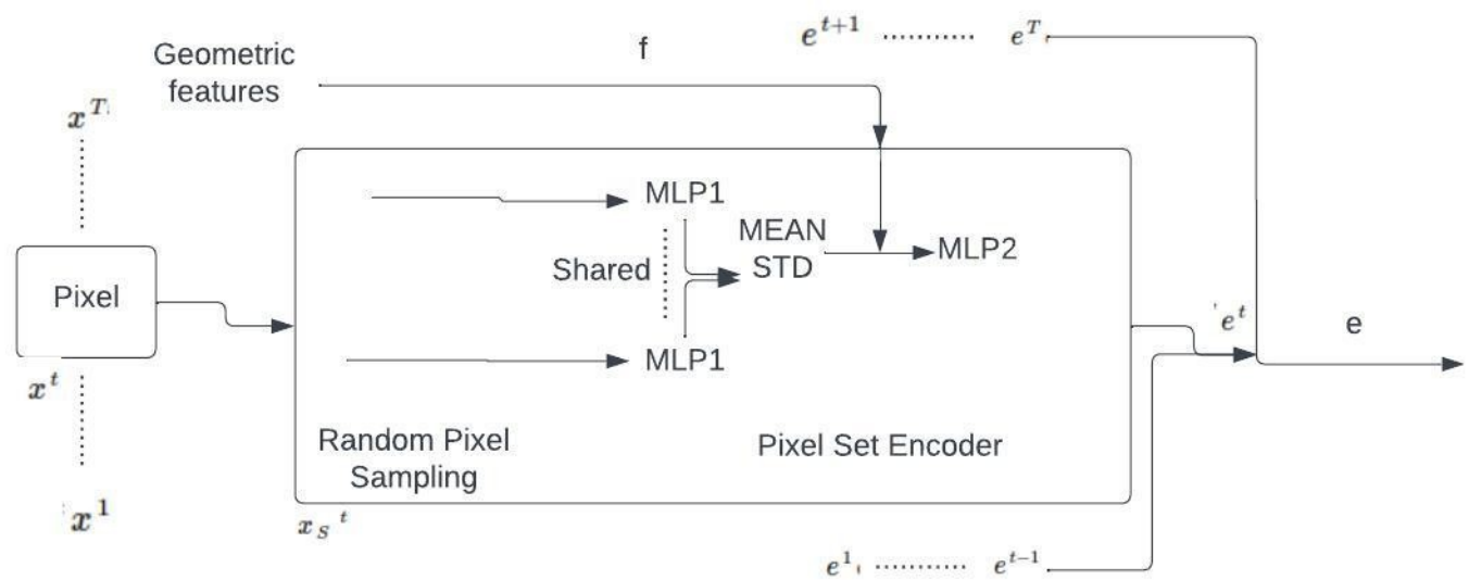
FIGURE 7. Pixel Set Encoder
