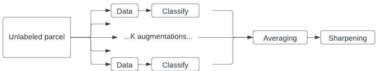
FIGURE 11. Mix Match Semi supervised algorithm
