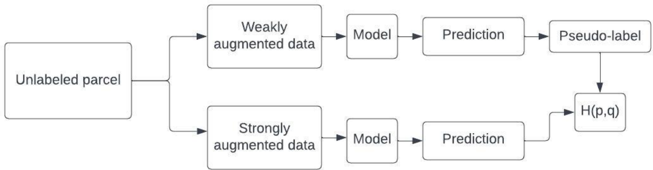
FIGURE 10. Fix Match Semi supervised algorithm
