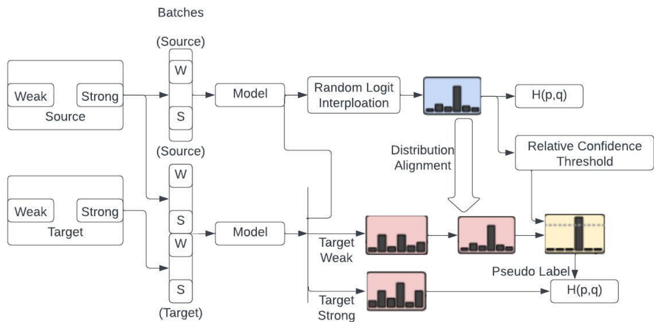
FIGURE 12. Ada Match Semi supervised algorithm
