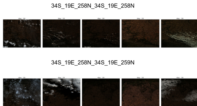
FIGURE 5. Sentinel 2 Five days time series plot
