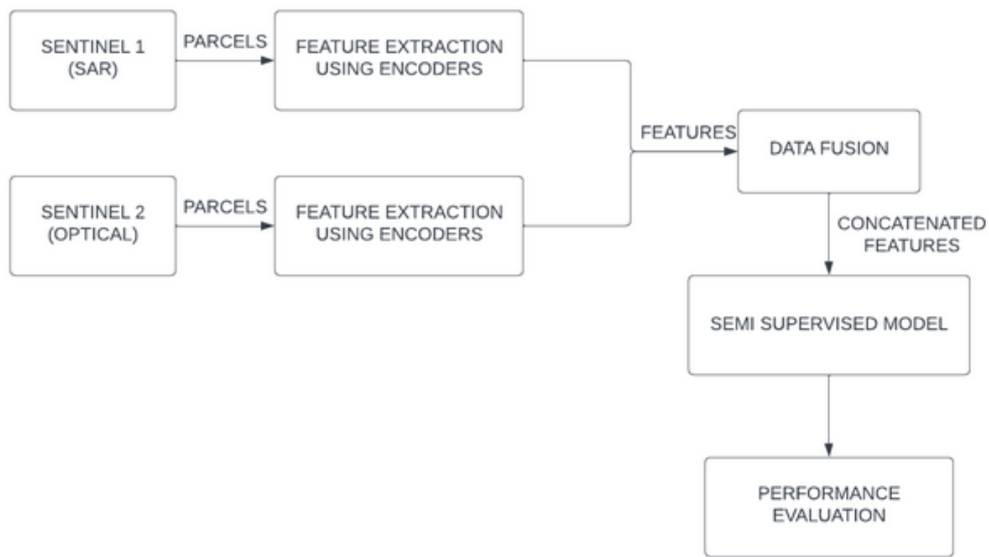
FIGURE 6. Methodology for the training process using Semi Supervised Learning
