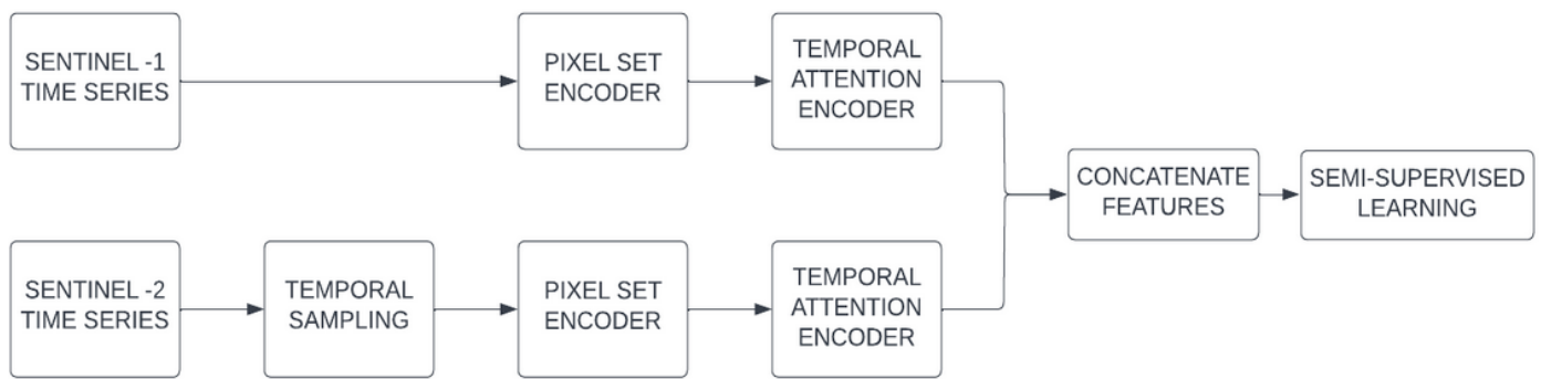
FIGURE 9. Layer level fusion architecture
